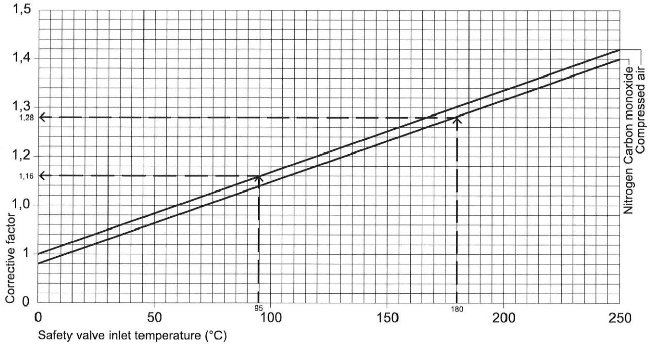
Fig. 2 Corrective factor in dependency of the temperature
